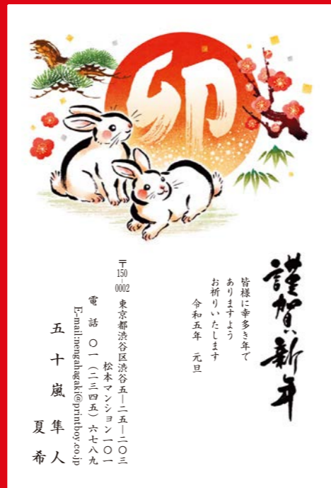
P-720 ★★★
